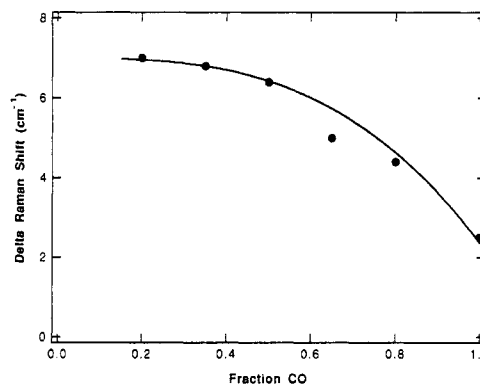
Figure 7. \Delta Raman shifts of CO compared with 2138.4 \text{ cm}^{-1} versus fraction of CO in mixtures of \text{N}_2 and CO at 7.2 GPa and \sim 1420 \text{ K} . The datum at 0.65 is near 6 GPa and is consequently slightly low compared with an empirical fit (—) of all of the CO and \text{N}_2 data. 16,18
